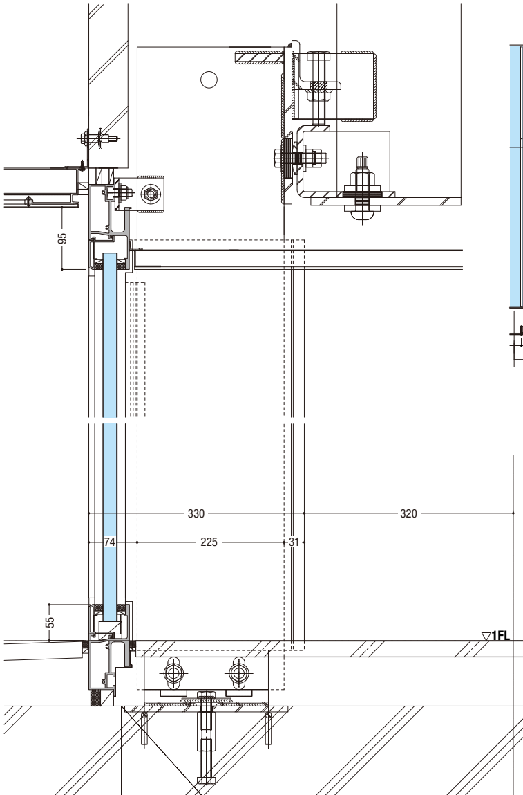
VERTICAL SECTION S=1/8
