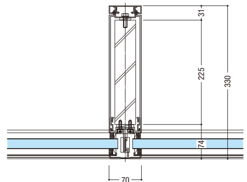
HORIZONTAL SECTION S=1/8
