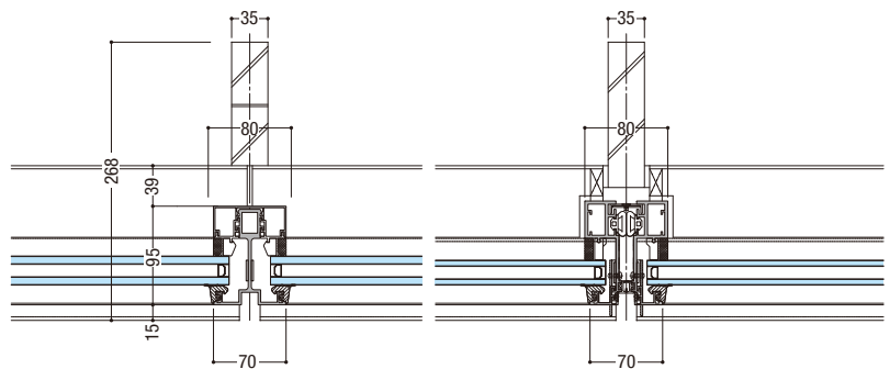
HORIZONTAL SECTION S=1/8
