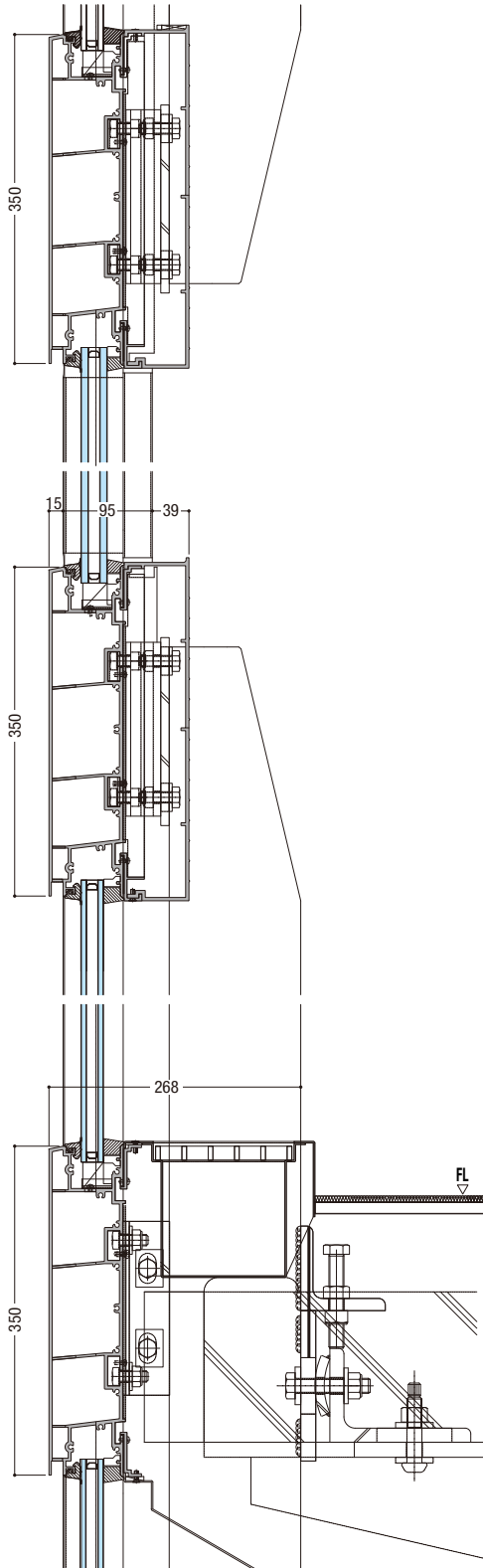
VERTICAL SECTION S=1/8
