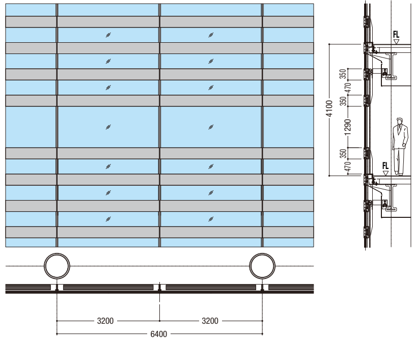
ELEVATION S=1/20
