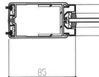
⑥85mm見付たて框 (St補強付)
