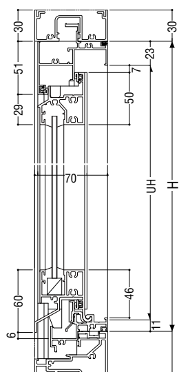
欄間内倒し排煙窓(70mm)
