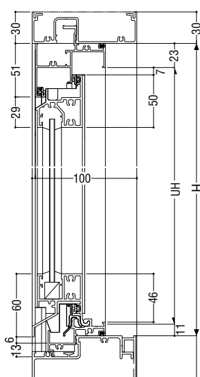
欄間内倒し排煙窓(100mm)
