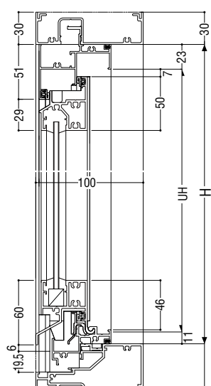
欄間内倒し排煙窓(100mm)
