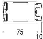
③ 85mm見付たて枠
