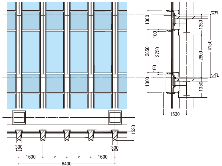
ELEVATION S = 1/150
